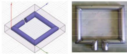
Fig.2: Square Loop (a) Numerical Design (b) Fabricated Prototype
