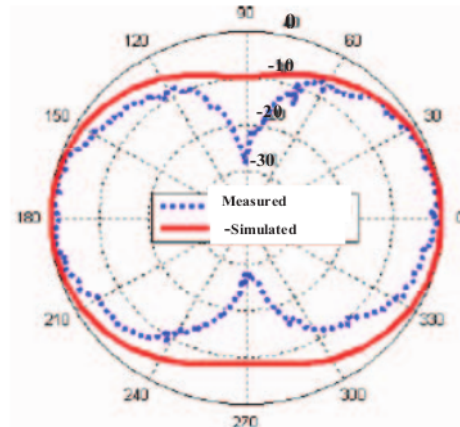
Fig.8 (b): Elevation pattern of circular plate loop structure
