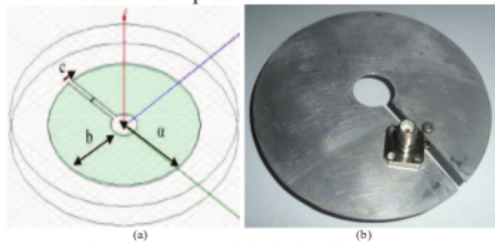
Fig.4: Disk Loop (a) Numerical Design (b) Fabricated Prototype
